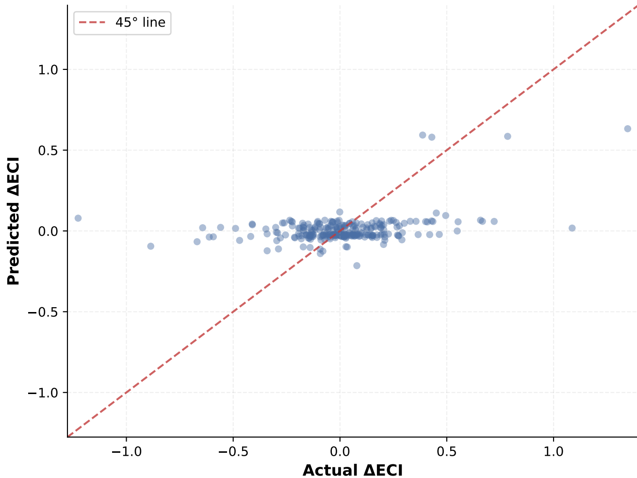
Random Forest — \Delta ECI | Test R^2=0.159 RMSE=0.2358
